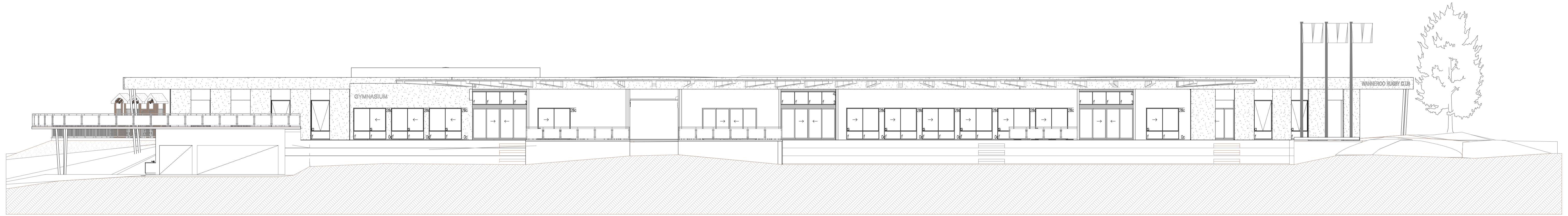
FRONT ELEVATION 1:150
